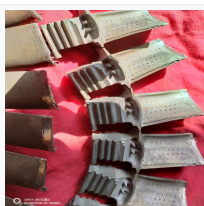
GE LM2500 1st-stage Turbine Blade (Single-Crystal Blade)
