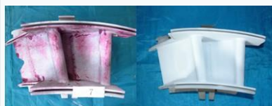
6B 1st-stage Nozzle
