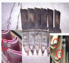
6B 1st-stage Turbine Blade
