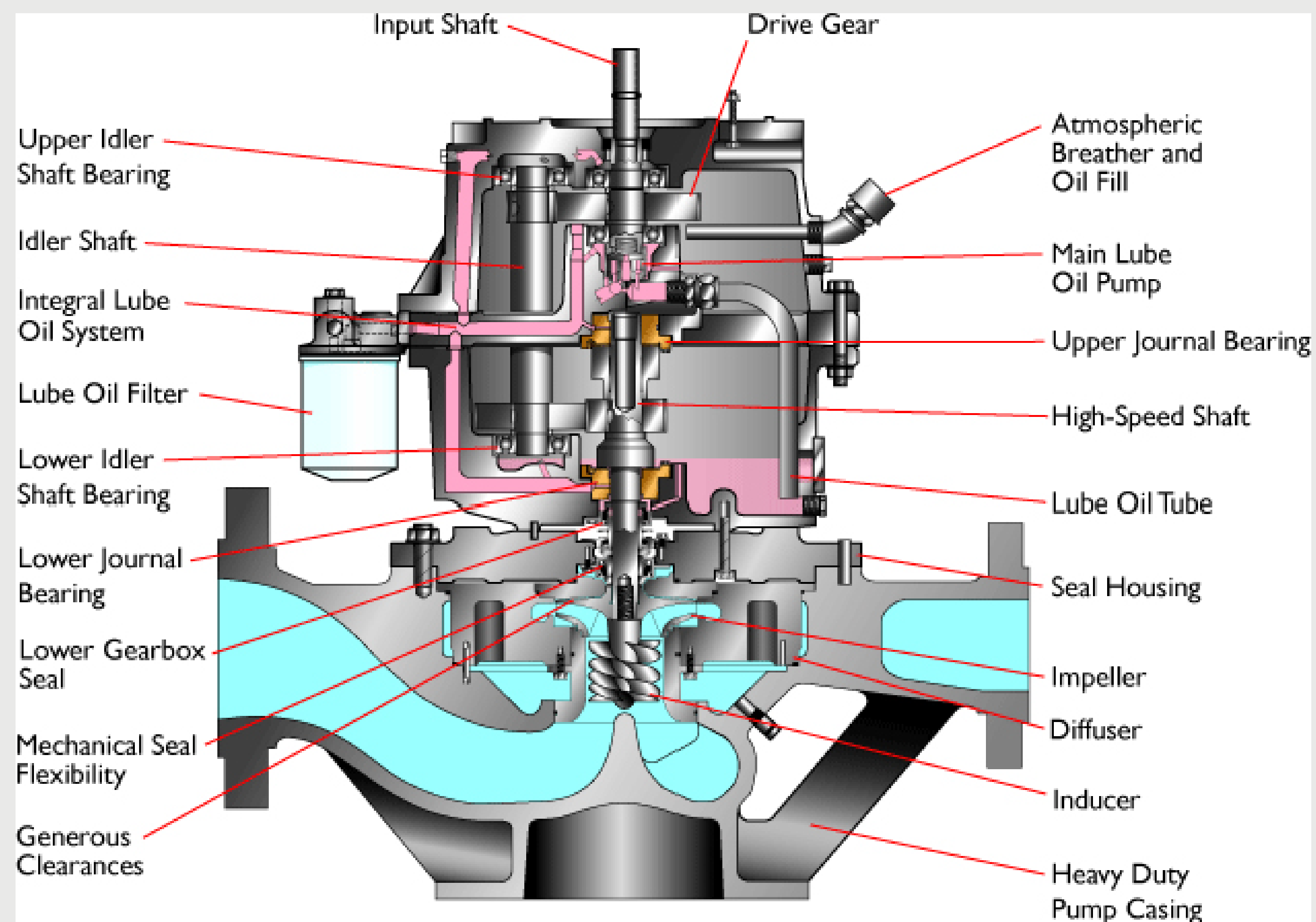
Sundyne LMV-313 Pump
