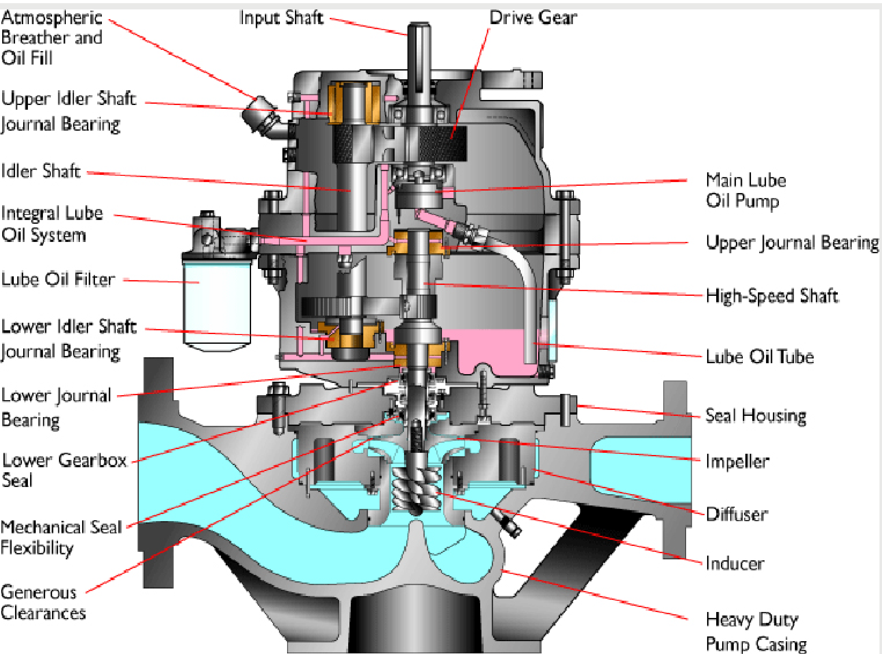
Sundyne LMV-333 Pump
