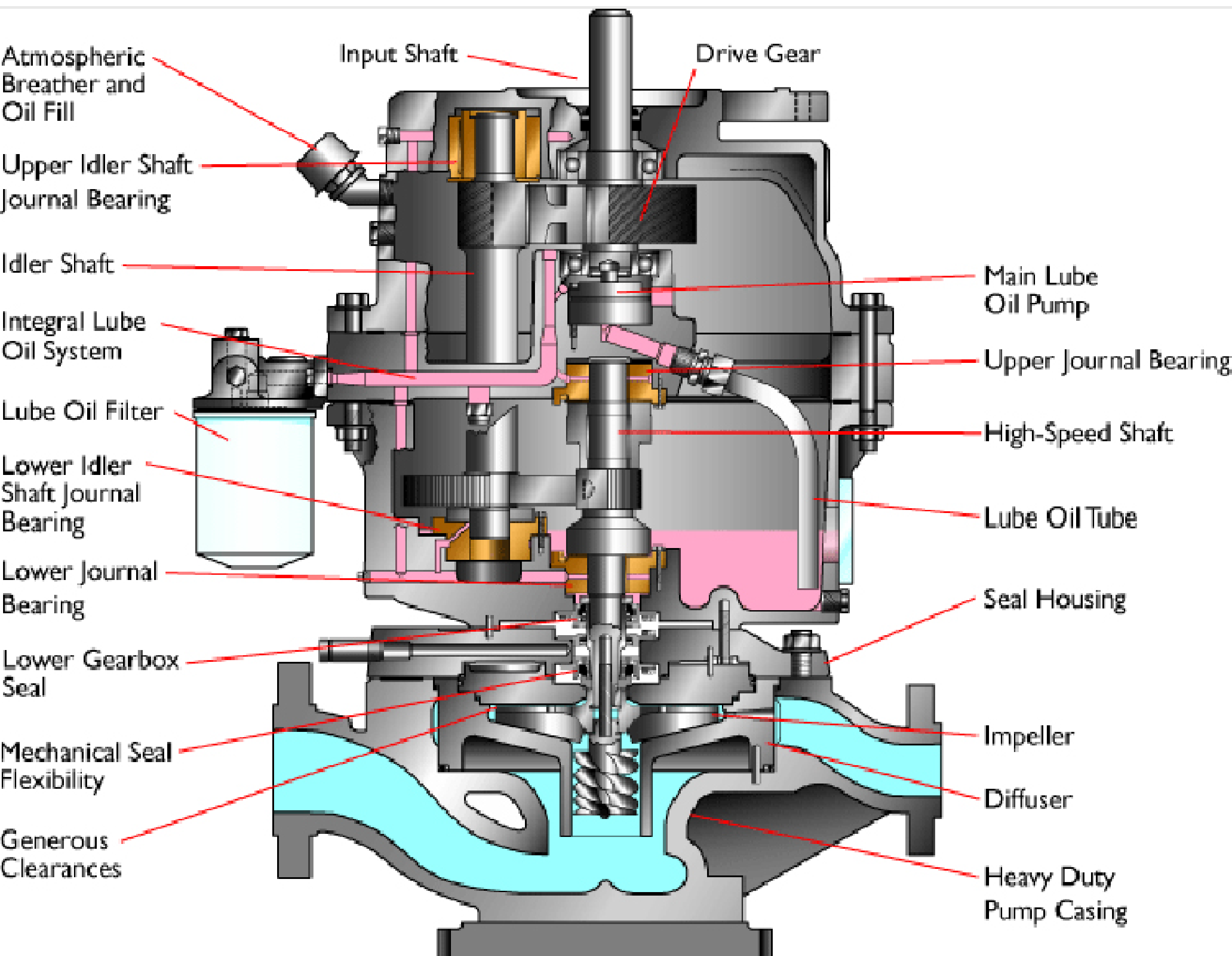
Sundyne LMV/BMP-331 Pump
