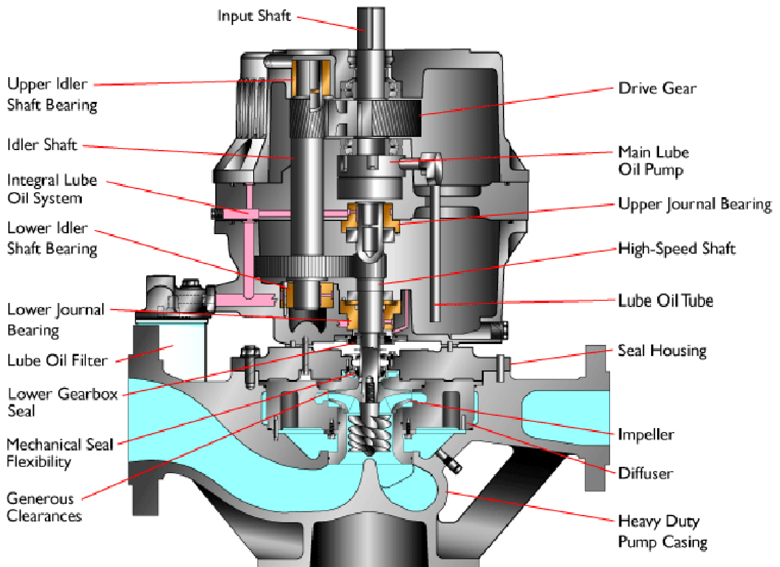
Sundyne LMV-343 Pump
