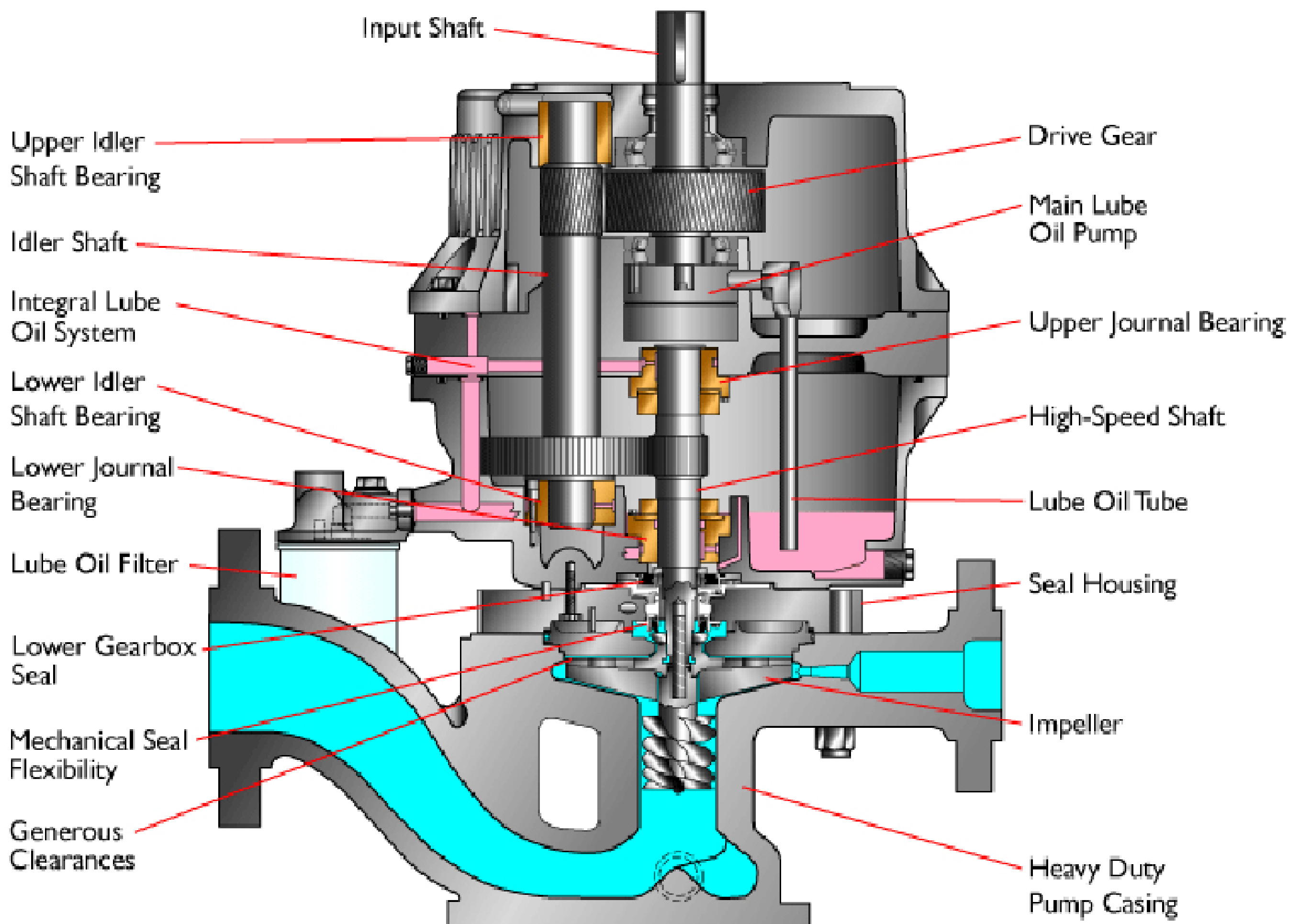
Sundyne LMV-346 Pump
