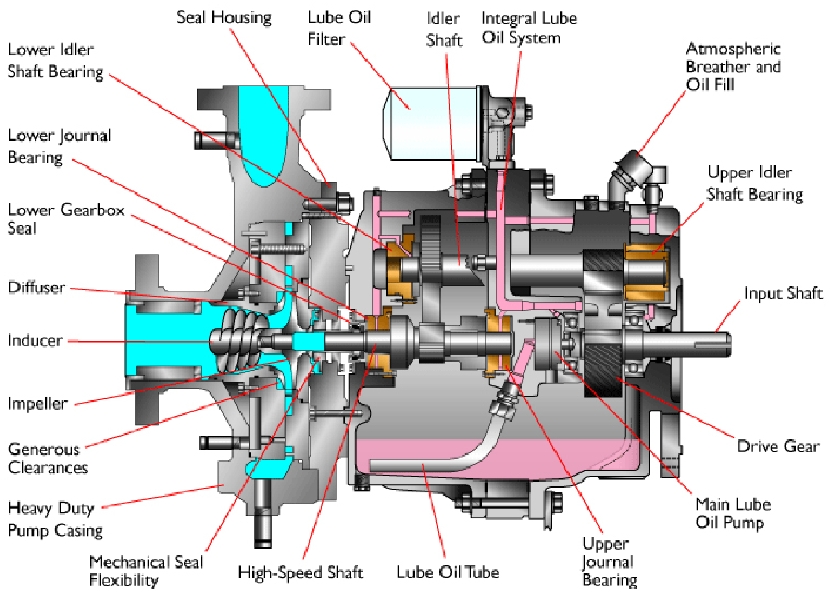
Sundyne BMP-338 Pump
