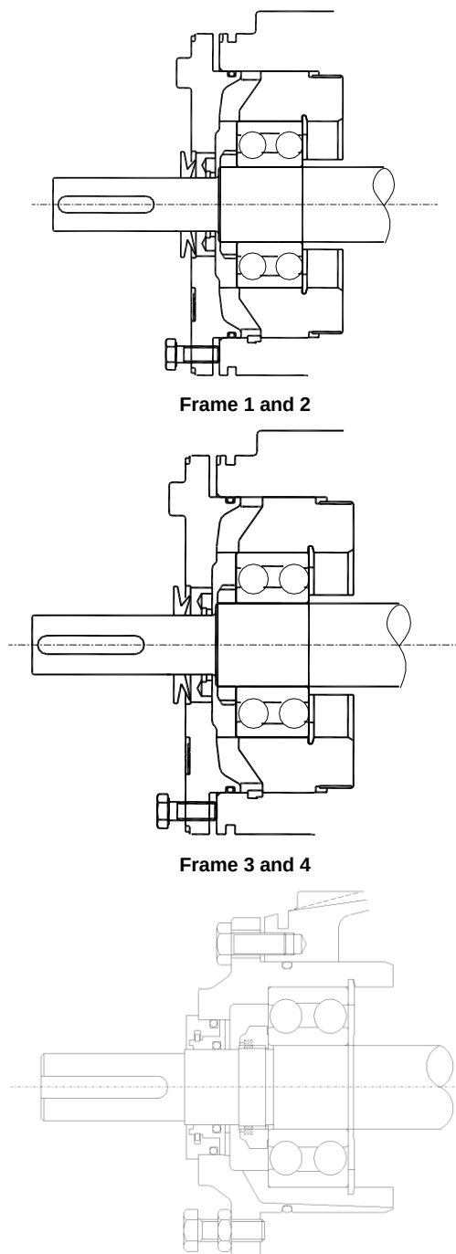
Frame 1 to 4 proprietary labyrinth/face seals (where fitted)
